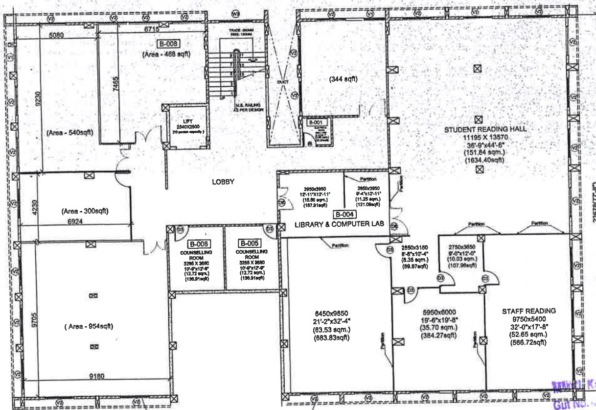
REVISED BASEMENT FLOOR PLAN
