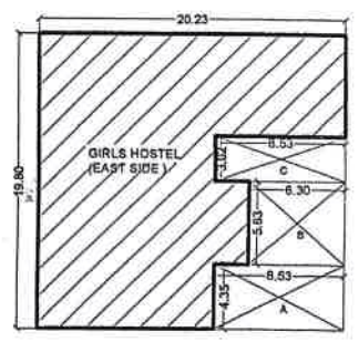
GIRLS HOSTEL (EAST SIDE) Forth floor
