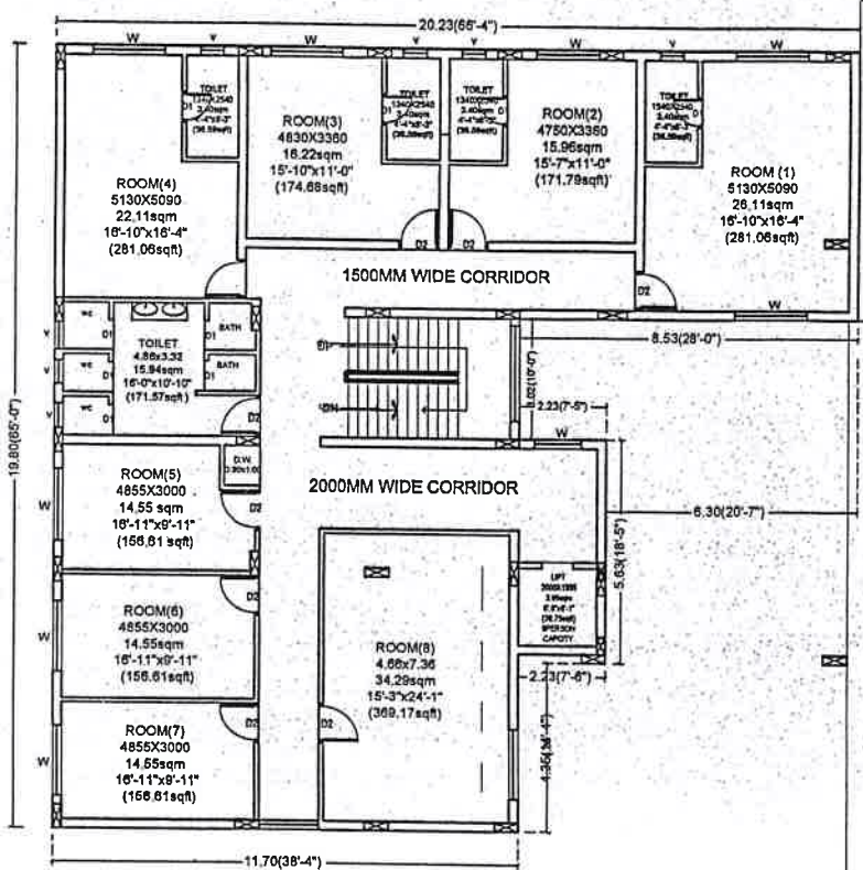
GIRLS HOSTEL (EAST SIDE)
