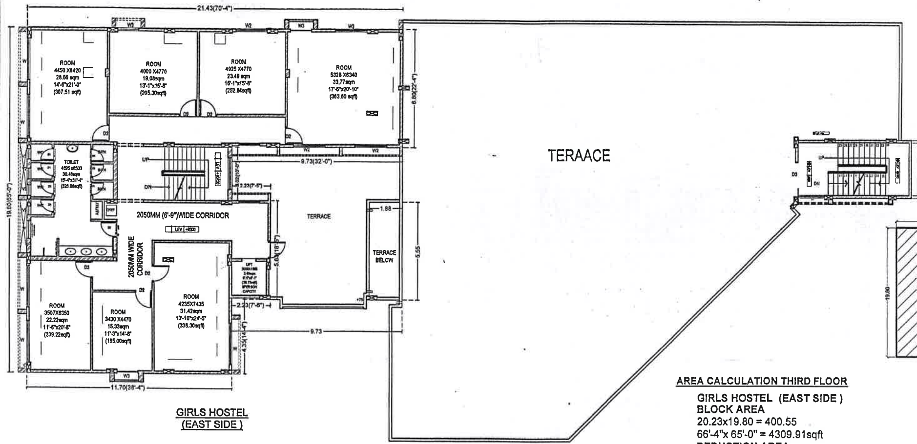
THIRD FLOOR
